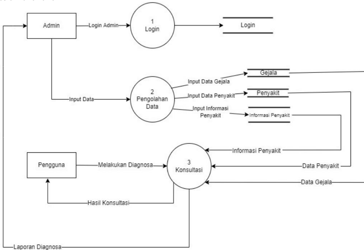
Gambar 4. DFD Level 1
