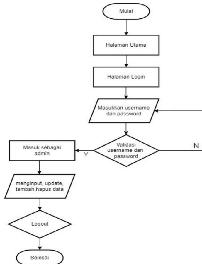
Gambar 1. Flowchart Admin
