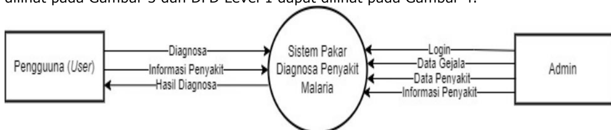
Gambar 3. DFD Level 0
