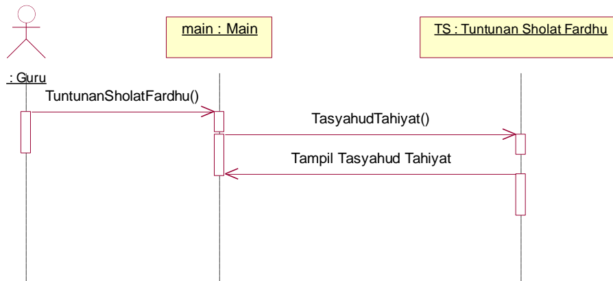
Gambar 4. Sequence Diagram bacaan tasyahud
